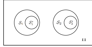
Fig. 8. Venn diagram, where \mathcal{S}_1, \mathcal{S}_2, \mathcal{S}_1^*, \mathcal{S}_2^* are defined as follows: Per run of proposed algorithm for RMOP, \mathcal{S}_1 and \mathcal{S}_2 are intermediate results such that \mathcal{S} = \mathcal{S}_1 \cup \mathcal{S}_2 , and \mathcal{S}_1 \cap \mathcal{S}_2 = \emptyset . Let \mathcal{S}_{\mathcal{A}}^*(\mathcal{S}) be the optimal removal from \mathcal{S} . Then \mathcal{S}_1^*, \mathcal{S}_2^* are defined such that \mathcal{S}_1^* = \mathcal{A}^*(\mathcal{S}) \cap \mathcal{S}_1 and \mathcal{S}_2^* = \mathcal{A}^*(\mathcal{S}) \cap \mathcal{S}_2 . By definition, \mathcal{S}_1^* \cap \mathcal{S}_2^* = \emptyset and \mathcal{S}_{\mathcal{A}}^*(\mathcal{S}) = \mathcal{S}_1^* \cup \mathcal{S}_2^* .
