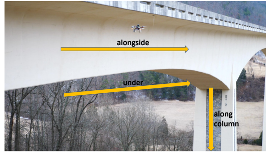
Fig. 2 Illustration of some useful navigation routines.
