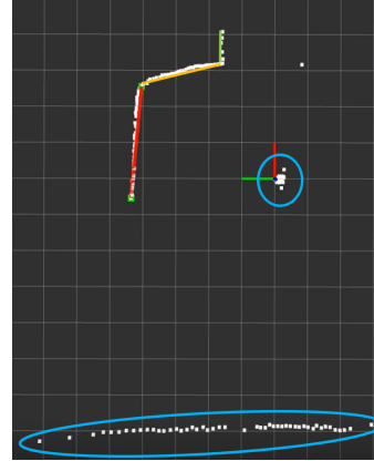
Fig. 7 Visualization (rviz) of filtered out points and extracted lines
