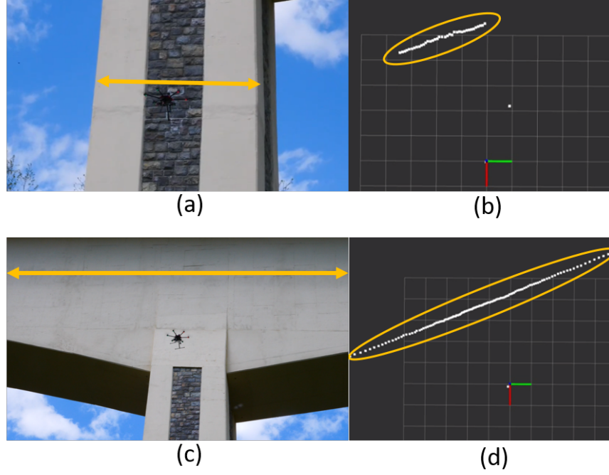
Fig. 9 Switching from column follow to girder follow.
