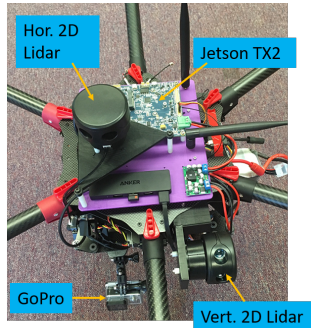
Fig. 1 UAV for bridge inspection.
