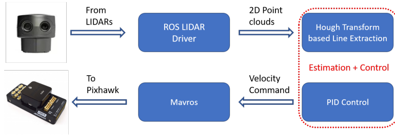
Fig. 4 Software architecture for autonomous navigation.
